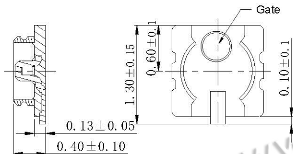
Detail-B Scale 4:1
