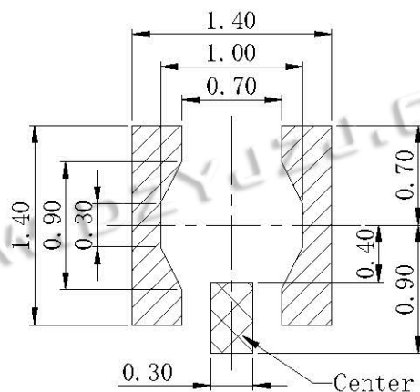
RECOMMENDED FOOTPRINT PATTERN TOP VIEW (TOLERANCE: ±0.05)
