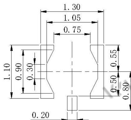
RECOMMENDED METAL MASK LAYOUT TOP VIEW (TOLERANCE: ±0.03), T=0.12
