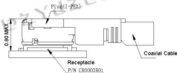
MATED VIEW
